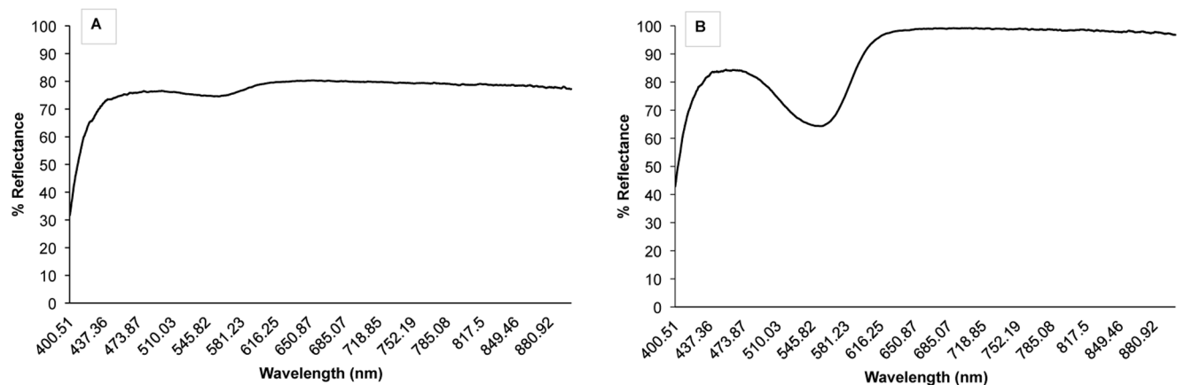
Figure 1. Reflectance spectra from a white staminate-phase flower, Pinkness Index (PI)=0.0764 (A) and a pink pistillate-phase flower, PI=0.4896 (B) of Saponaria officinalis . doi:10.1371/journal.pone.0093615.g001
